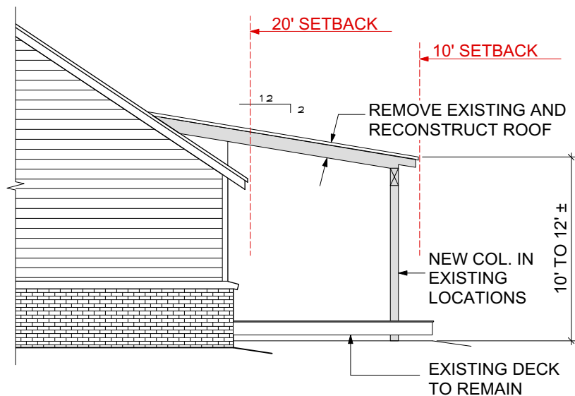
North Elevation
