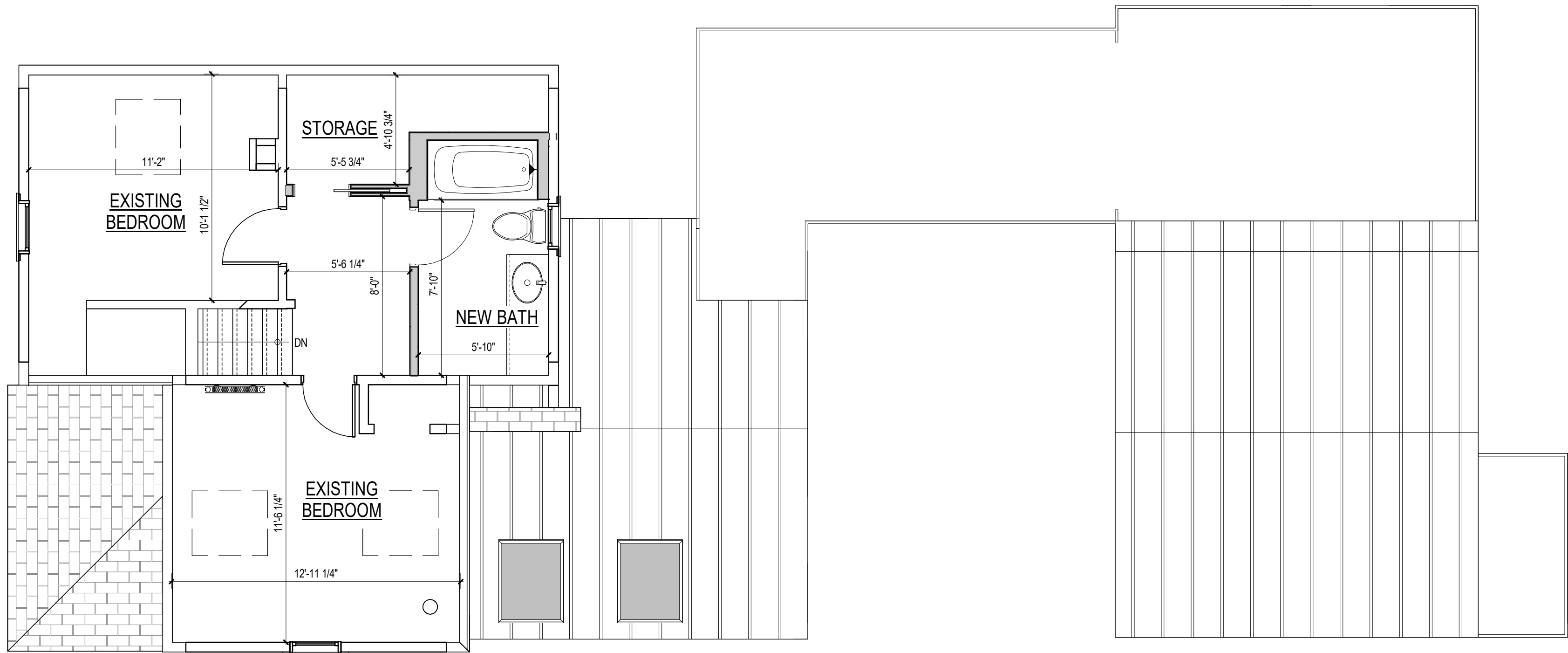
1 A.2 UPPER LEVEL FLOOR PLAN 1/4" = 1'-0"
