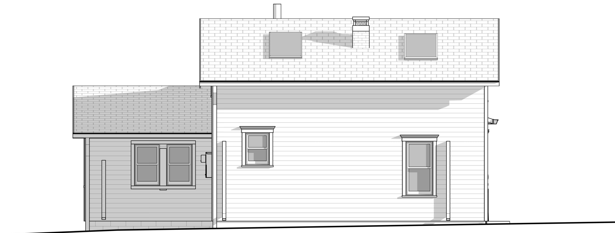
1 A.5 1/4" = 1'-0" EXISTING NORTH ELEVATION
