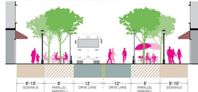
PROPOSED MAIN STREET SECTION
