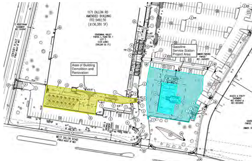
Areas of Proposed Improvements
