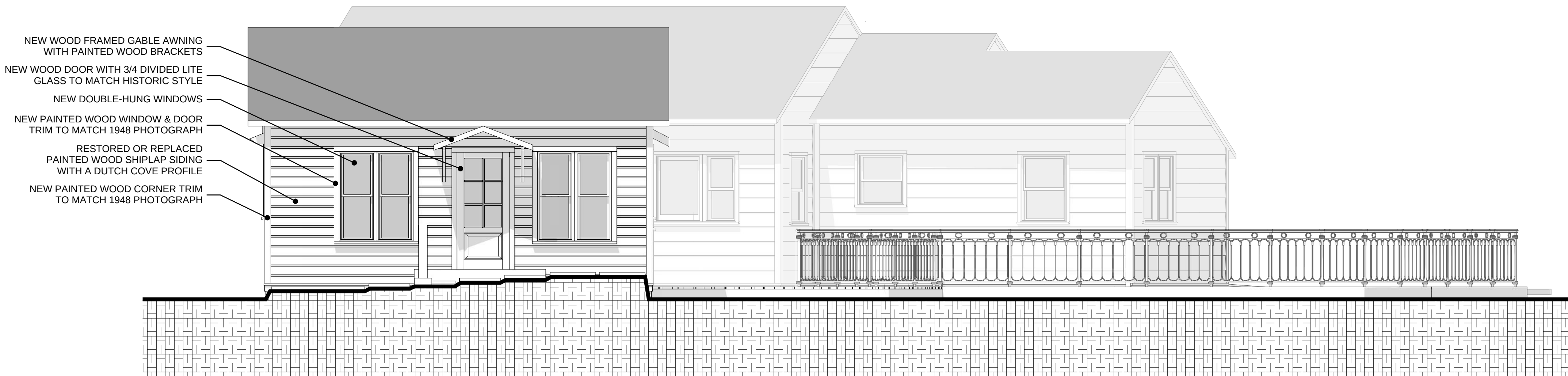
1 SOUTH ELEVATION
