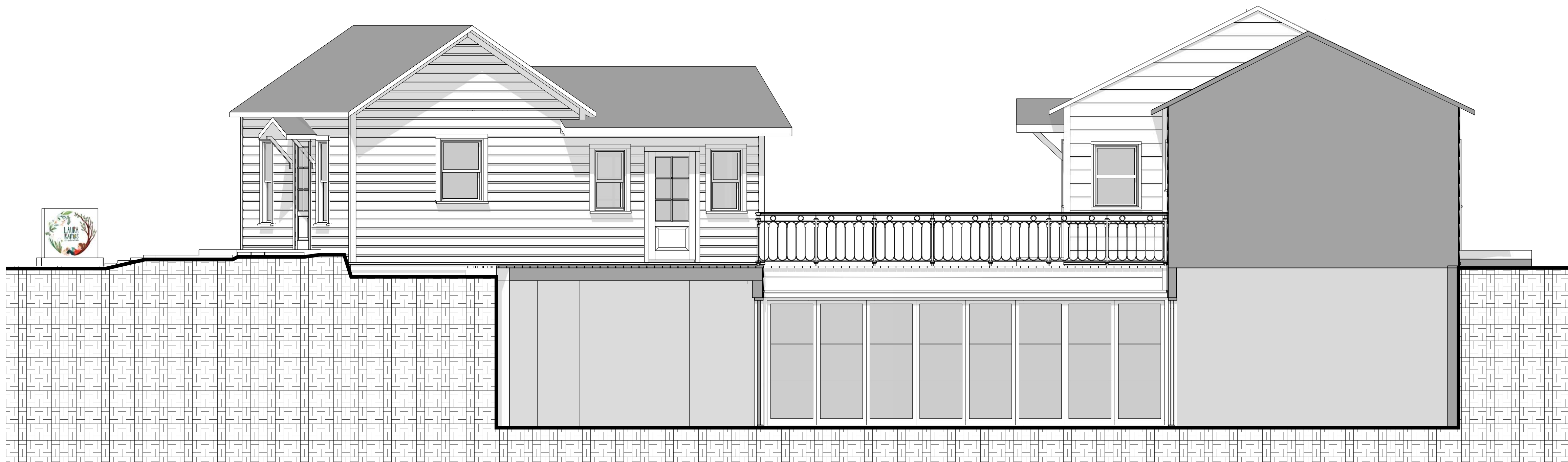
2 EAST SECTION
